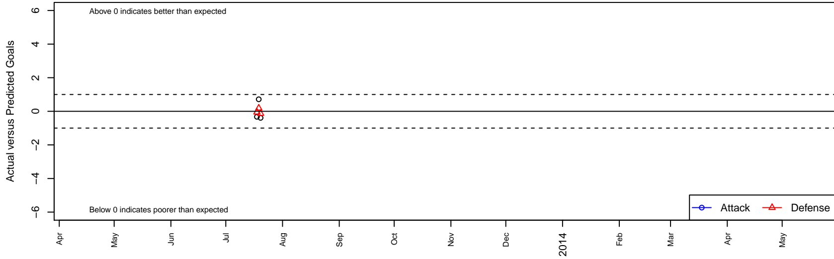
Whitecaps B96 Dots are actual minus expected GF (blue circles) and GA (red triangles). Blue line is smoothed change in attack strength. Red is smoothed change in defense strength.
